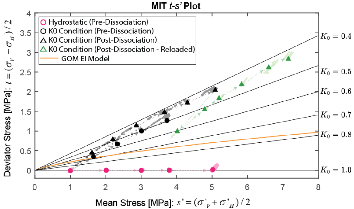
Figure 1-8: Stress path of experiments performed on Core 6FB2. At each sample point, permeability was measured. Initially the experiments were run within the hydrate stability zone under increasing isostatic stresses (pink circles). Then the sample was unloaded and reloaded (still within the hydrate stability zone) under uniaxial strain conditions (black circles). Then the sample was dissociated under constant effective stress. Then the sample was reloaded uniaxially (black triangles and green triangles). The K_0 coefficient (the ratio of lateral to vertical effective stress ( K_0 = \frac{\sigma_{H'}}{\sigma_{v'}} )) is between 0.4 and 0.5. Dissociation of hydrate does not significantly change the K_0 coefficient (the black circles and the black triangles follow a similar path).
