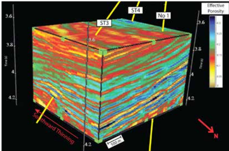
POROSITY ESTIMATION FROM 3D SEISMIC AND WELL LOG DATA AIDS IN LOCATING AND PREDICTING THE NATURE OF UNDERGROUND RESOURCES. THE EXAMPLE SHOWN HERE IS FROM THE MARCO POLO FIELD, GULF OF MEXICO. CREDIT: G. RUSSEL YOUNG AND MRINAL SEN
