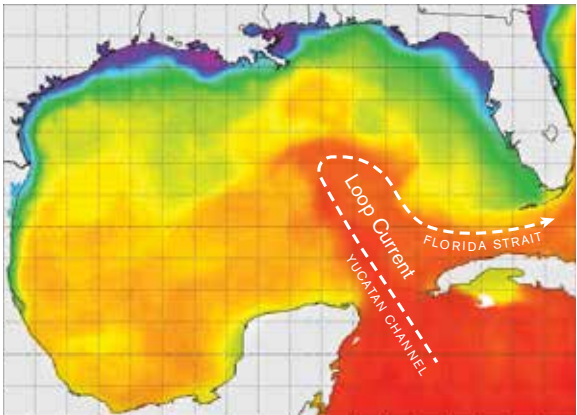
THE LOOP CURRENT STUDY WILL INVESTIGATE HOW WATER FLOW INTO AND OUT OF THE GULF OF MEXICO HAS CHANGED THROUGH TIME AND HOW IT RELATES TO REGIONAL CLIMATE. CREDIT: CHRIS LOWERY
